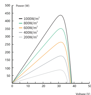
Power-Voltage Curve(445W)
